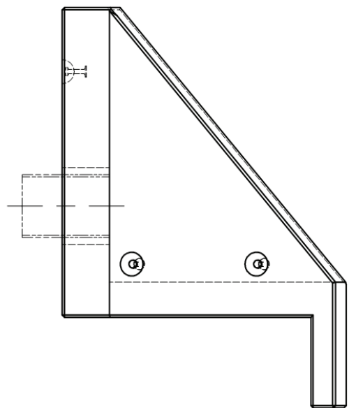
Side Elevation View
