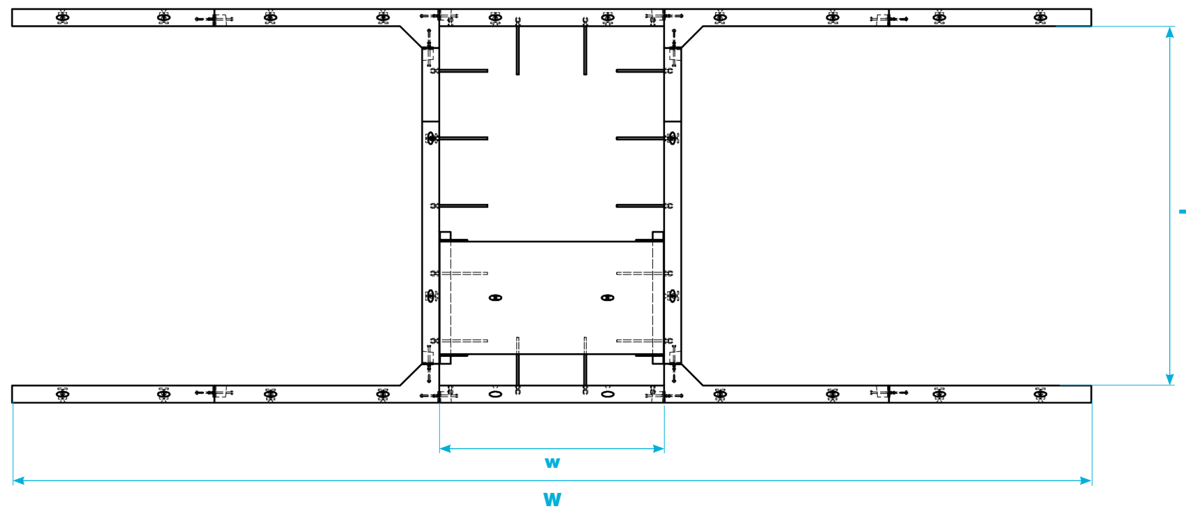
Plan View
